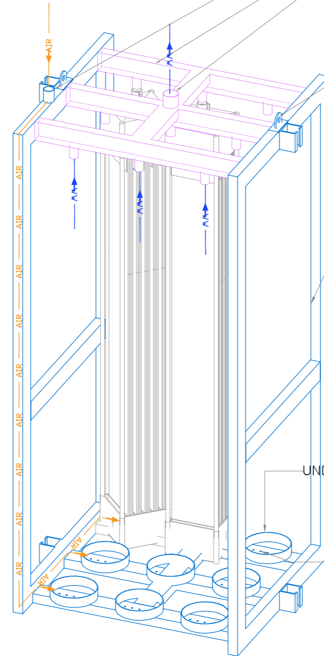
ISOMETRIC
