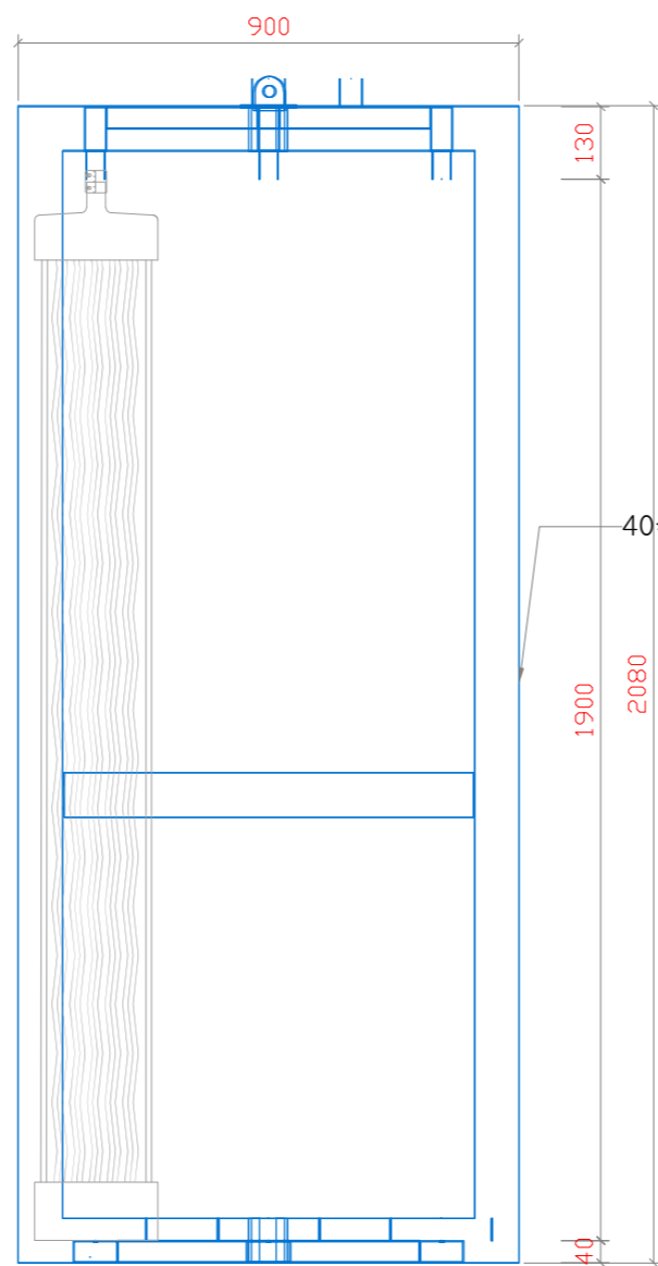
SECTION 2-2
