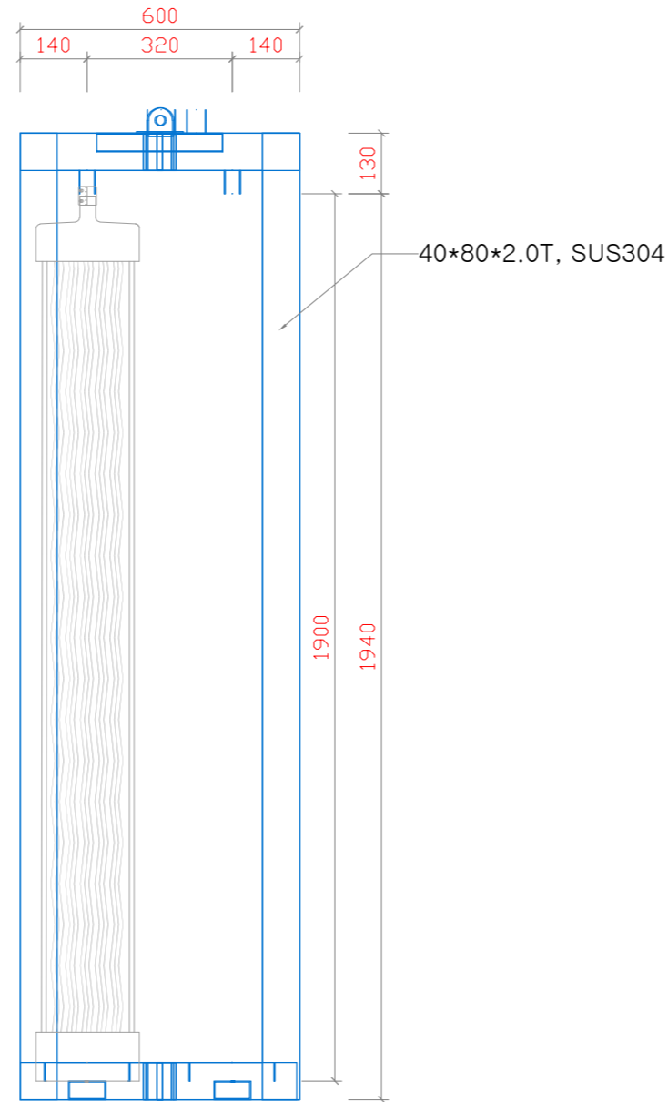
SECTION 2-2
