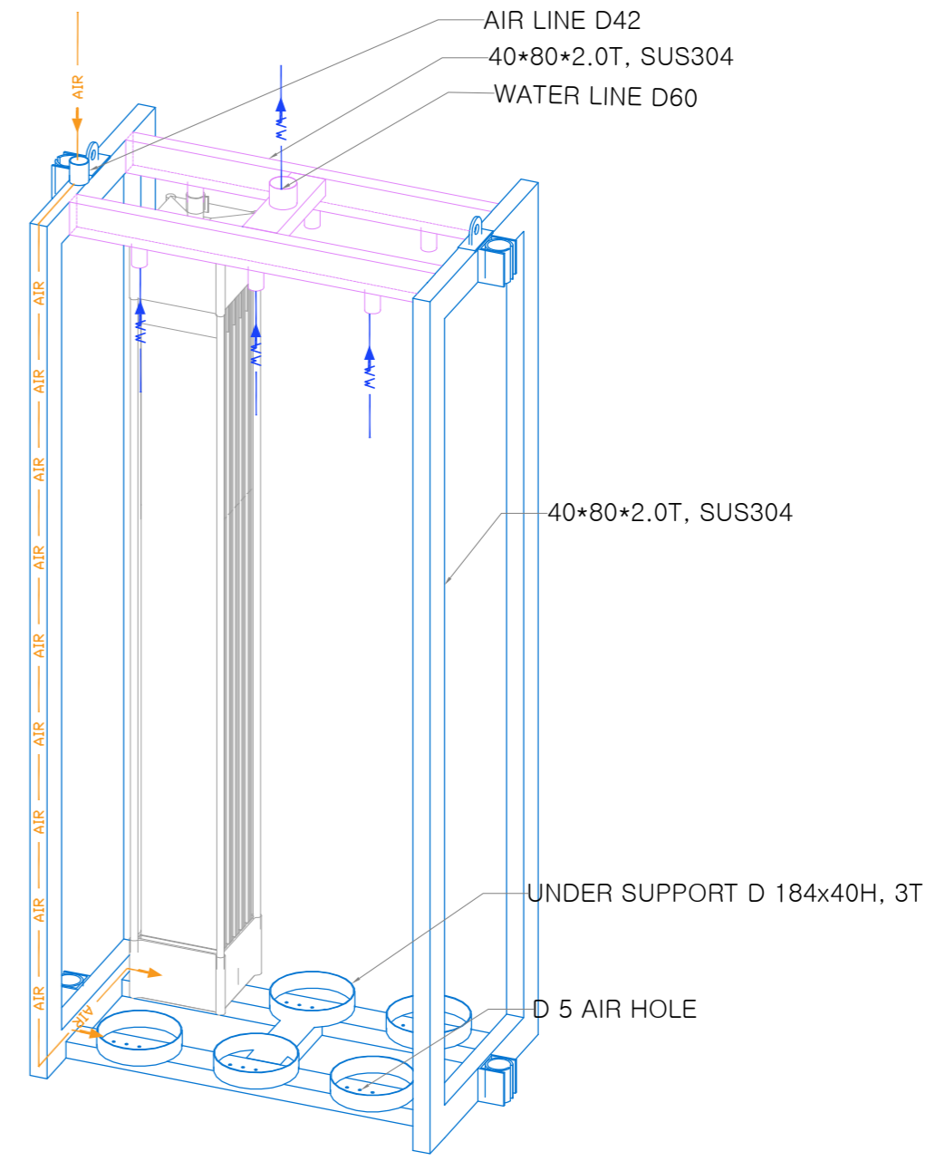
ISOMETRIC
