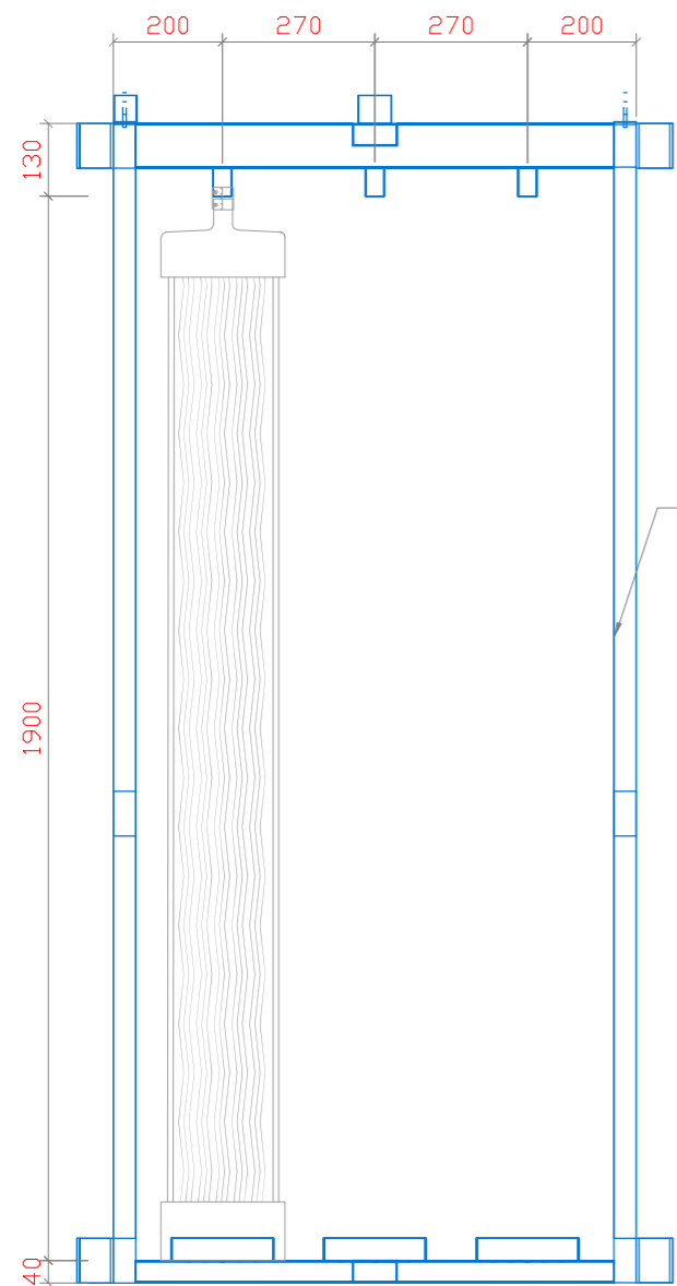
SECTION 1-1
