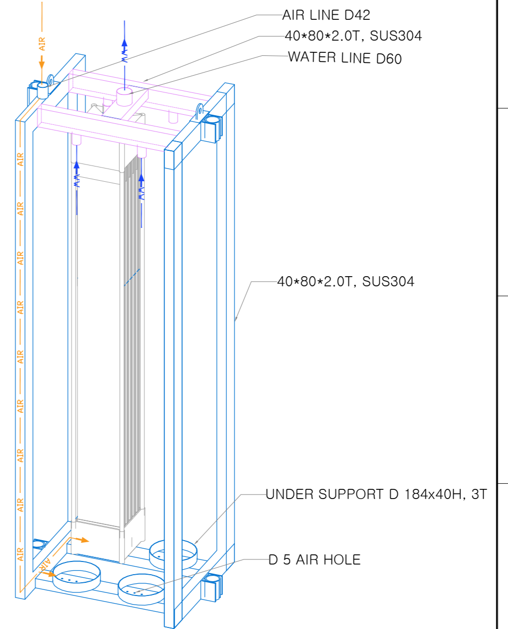
ISOMETRIC
